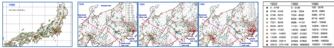
Figure 33. Changes in population distribution superposed on road network (central Japan).
