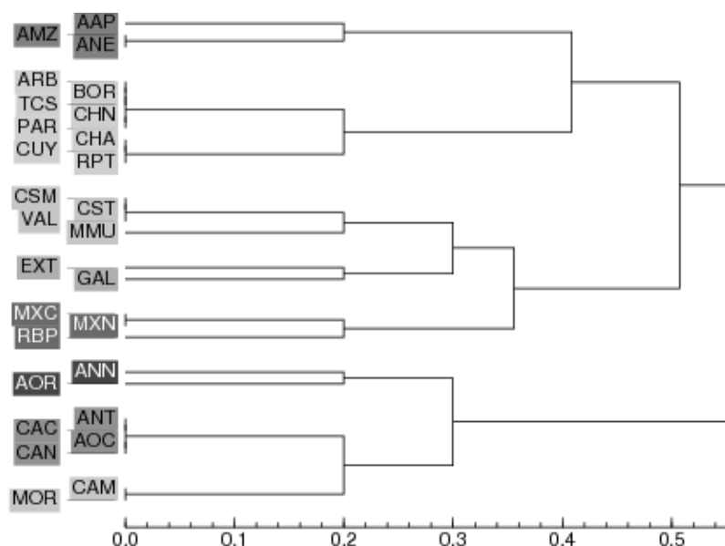
Figure 3. Dendrogram of eight clusters using /r/-assibilation
